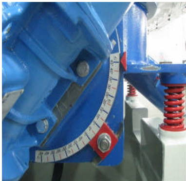
MOTOR ADJUSTMENT
